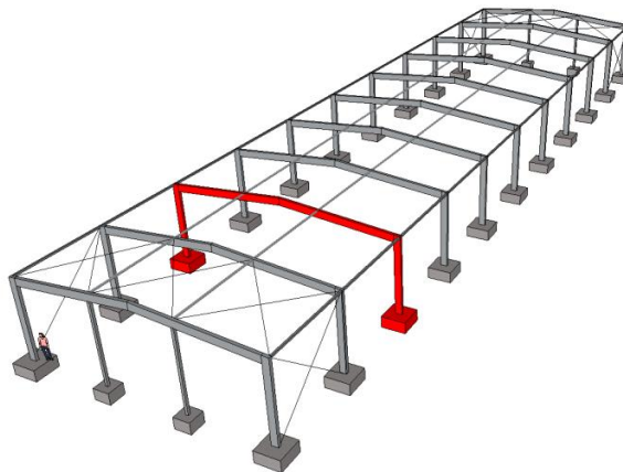
Figure 1: Isometric view of a single storey buildings structural system with the regarded functional unit, a basic frame structure
