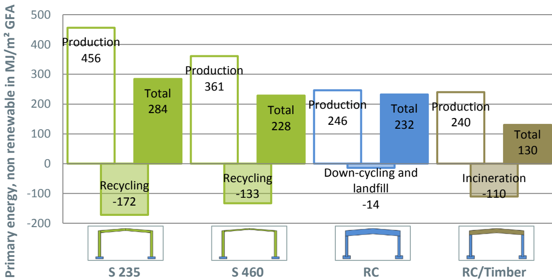
Figure 11: Non renewable primary energy for the Product Stage (A1-A3) and separately Benefits & Loads (D) from recycling (steel), incineration (timber) or rubble processing combined with an replacement of gravel (concrete) in MJ per m² gross floor area
